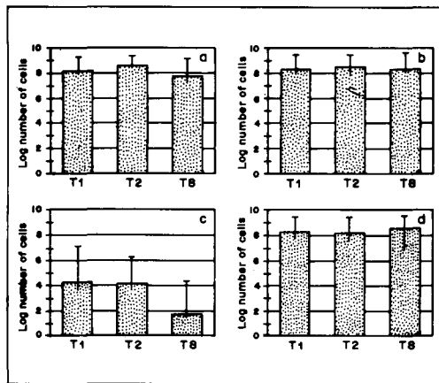
Fig. 1. MPN of 2, 4-D degraders and total viable comb (or total heterotroph) before and after 2, 4-D selection (a) Total viable count before 2, 4-D selection, (b) Total viable count after 2, 4-D selection, (c) MPN or 2, 4-D degraders before 2, 4-D selection (d) MPN of 2, 4-D degraders after 2, 4-D selection.
