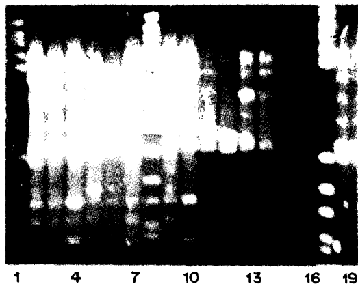
Fig. 3. Community ADRA pattern of soil treatments before and after 2, 4-D addition. Lanes 1, 8, 16, and 17 are marker DNA V; Lanes 2 to 4, T1 before 2, 4-D addition, Lanes 5 6 T1 after 2, 4-D addition, Lanes 7, 9, 10, T2 before 2, 4-D; Lanes 11 to 12, T2 after 2, 4-D, Lanes 13 to 15, T8 before 2, 4-D, and lanes 18 and 19, T8 after 2, 4-D.
