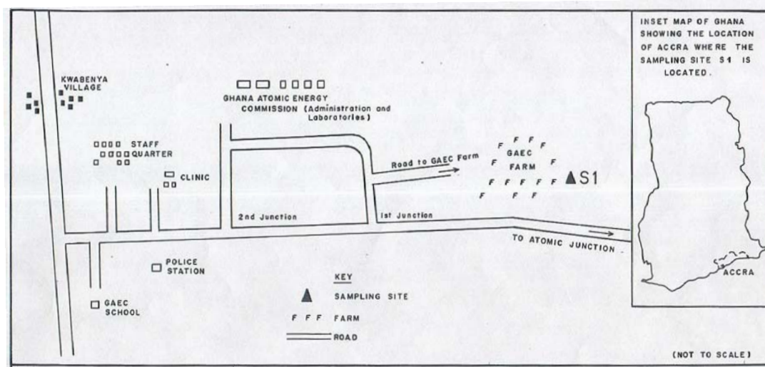
Fig. 1. A sketch map of a section of GAEC showing the sampling site S1
