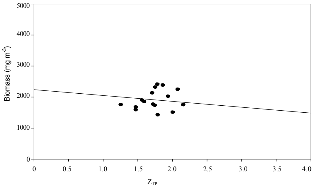
Fig. 11. Phytoplankton biomass as a function of variations in total phosphorus concentration ( Z_{TP} ) of Lake Bosomtwe (Ghana); November 2004 – October 2006.
