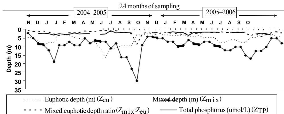
Fig. 1. Temporal variation in euphotic depth ( Z_{eu} ), mixed layer depth ( Z_{mix} ), mixed layer:euphotic depth ratio ( Z_{mix}:Z_{eu} ), and total phosphorus concentration ( Z_{TP} ) of Lake Bosomtwe (Ghana) from November 2004 to October 2006.
