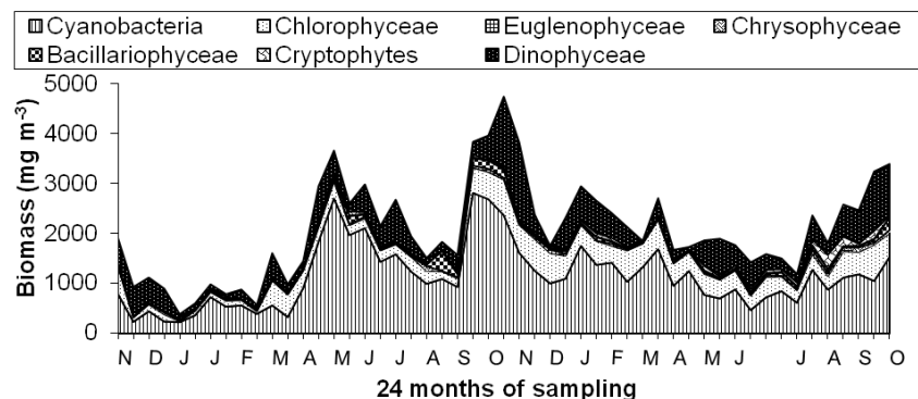
Fig. 6. Temporal variation in wet weight biomass of phytoplankton of Lake Bosomtwe (Ghana) showing the contribution of the different groups of phytoplankton from November 2004 to October 2006.
