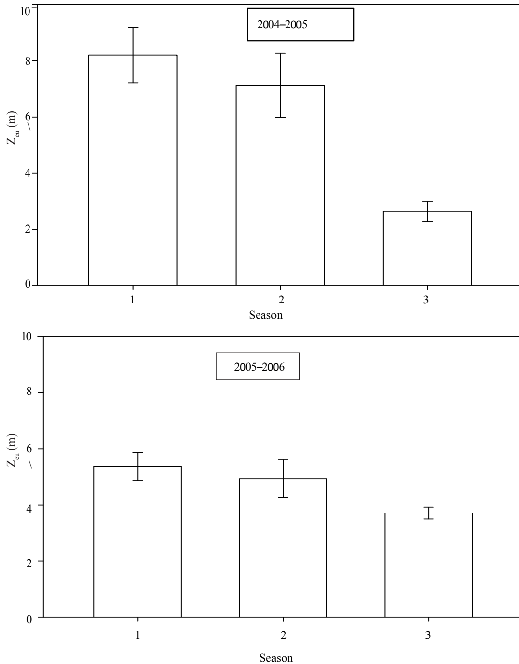
Fig. 3. Seasonal variation in the euphotic ( Z_{eu} ) (mean \pm s.e) depth of Lake Bosomtwe (Ghana) from 2004-2005 and 2005-2006 sampling periods respectively. (1 = stratified period; 2 = mixing period; 3 = restratifying period).
