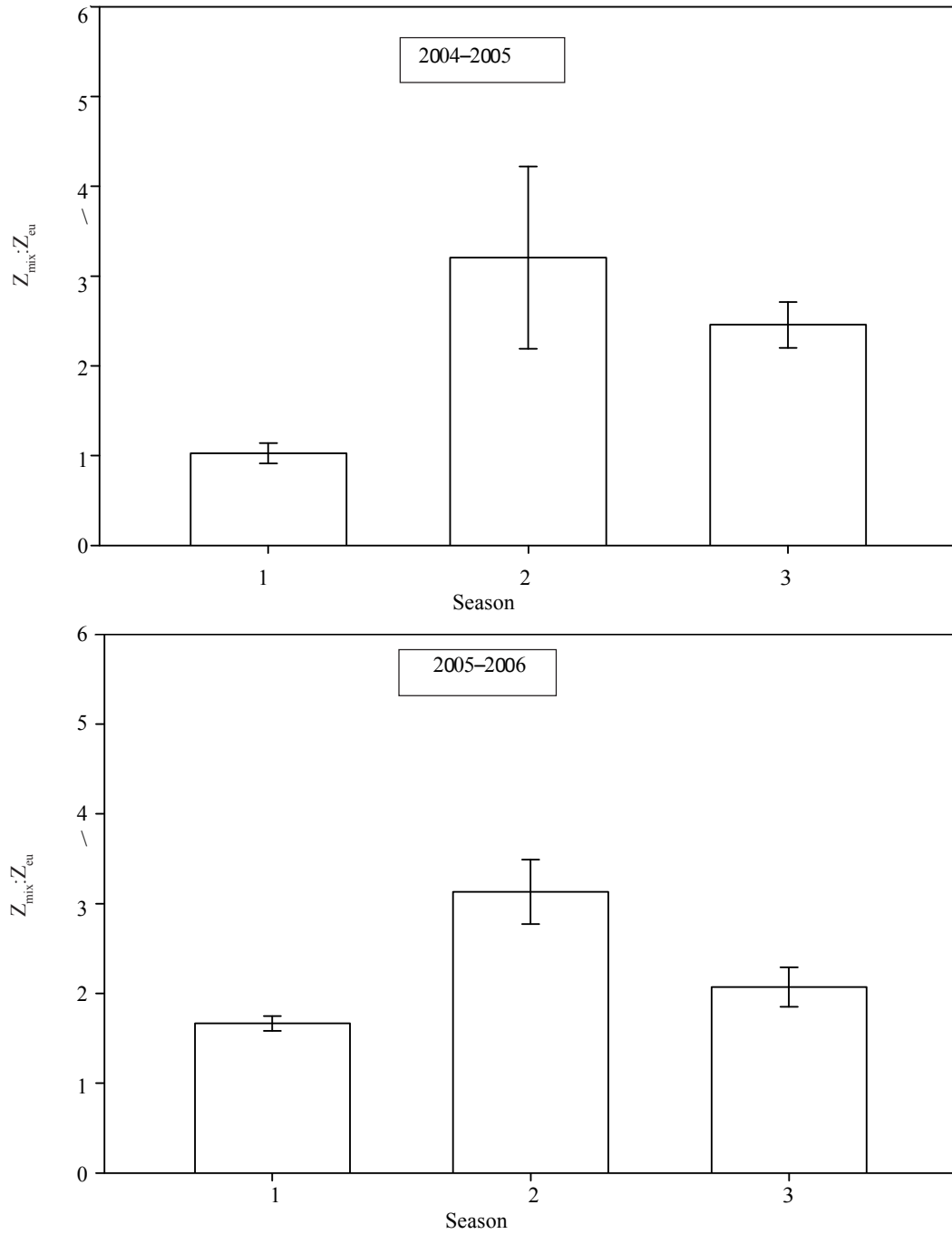
Fig. 4. Seasonal variation in the mixed layer:euphotic depth ( Z_{mix}:Z_{eu} ) (mean \pm s.e) of Lake Bosomtwe mixing period; 3 = restratifying period).
