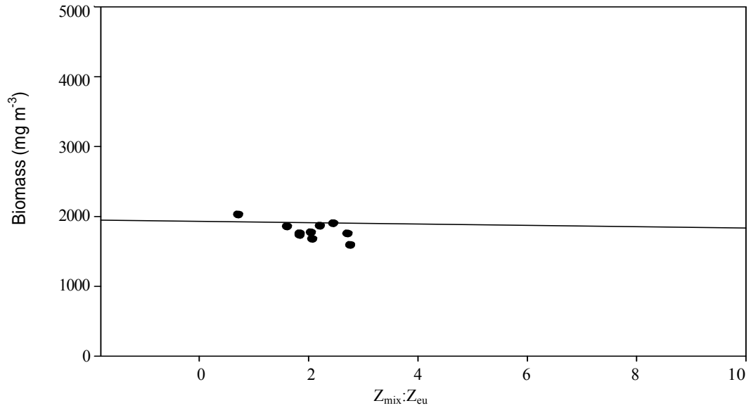
Fig. 10. Phytoplankton biomass as a function of variations in the mixed layer:euphotic depth ratio depth ( Z_{mix}:Z_{eu} ) of Lake Bosomtwe (Ghana); November 2004 – October 2006.
