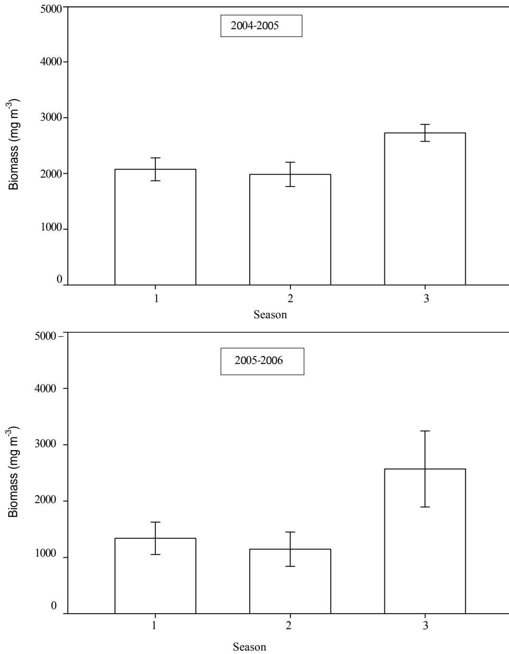
Fig. 7. Seasonal variation phytoplankton wet weight biomass measure (mean \pm s.e) of Lake Bosomtwe (Ghana) from 2004-2005 and 2005-2006 sampling periods respectively. (1 = stratified period; 2 = mixing period; 3 = restratifying period).
