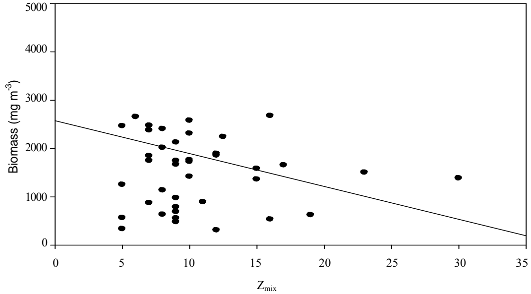
Fig. 8. Phytoplankton biomass as a function of variations in mixed layer depth ( Z_{mix} ) of Lake Bosomtwe (Ghana); November 2004 – October 2006.
