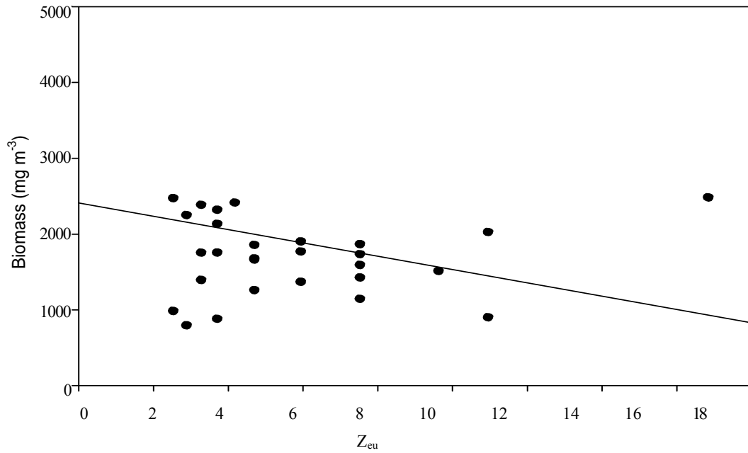
Fig. 9. Phytoplankton biomass as a function of variations in euphotic depth ( Z_{eu} ) of Lake Bosomtwe (Ghana); November 2004–October 2006.
