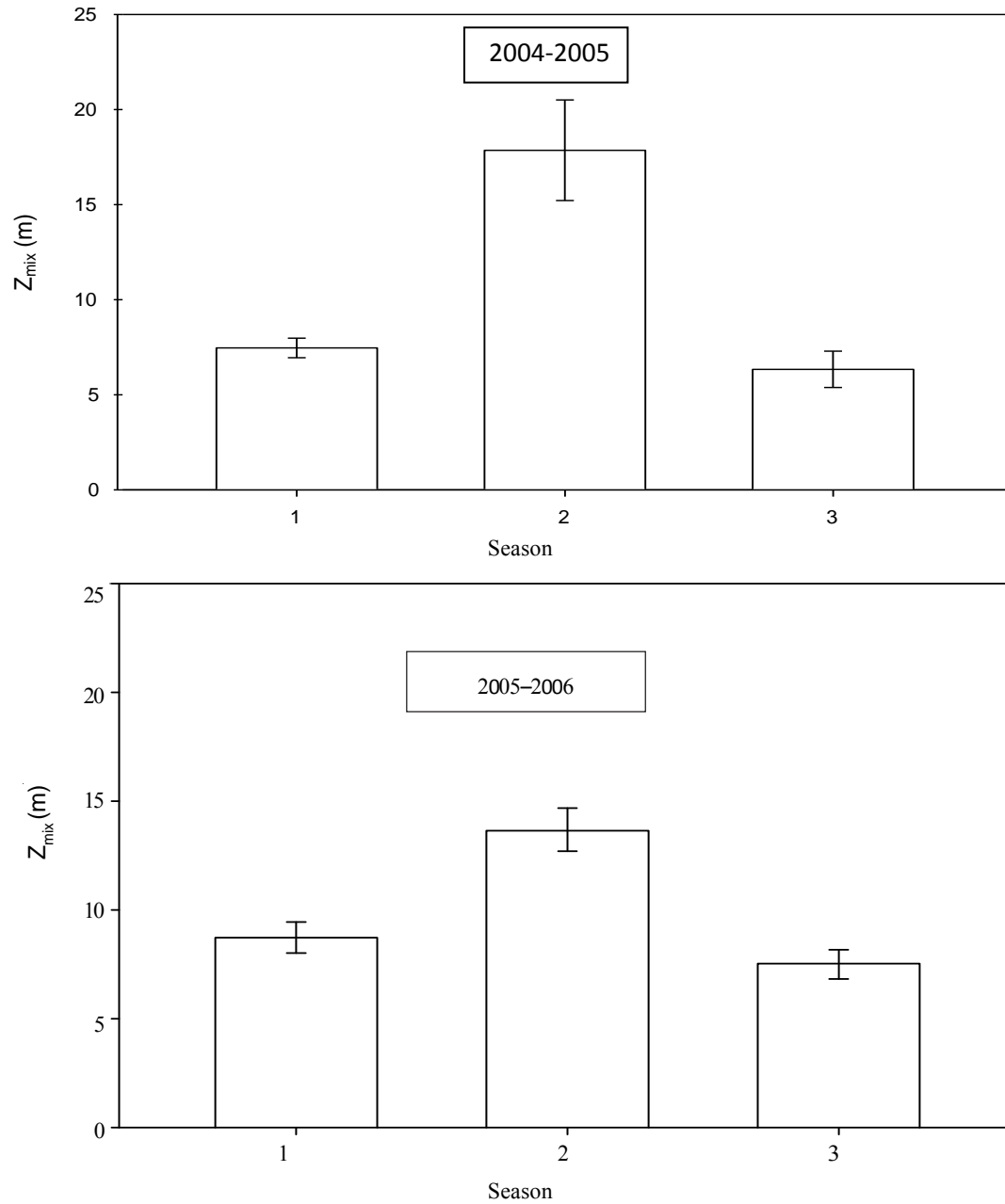
Fig. 2. Seasonal variation in depth of mixed water layer ( Z_{mix} ) (mean \pm s.e) of Lake Bosomtwe (Ghana) from 2004-2005 and 2005-2006 sampling periods respectively. (1 = stratified period; 2 = mixing period; 3 = restratifying period).
